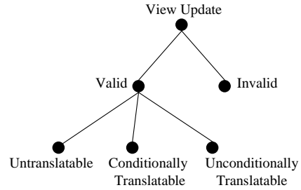
Fig. 8. The partition of view update domain \mathcal{U}^V
