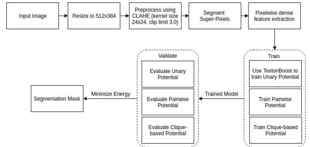
FIGURE 4: AHRF implementation and workflow
