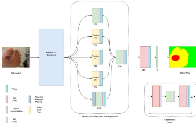
FIGURE 7: Architecture of DeepLabV3.
