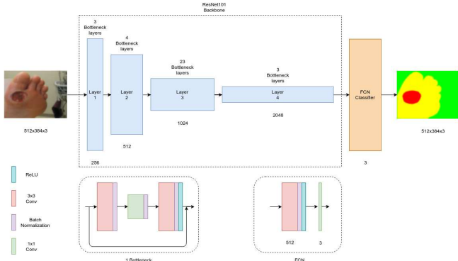
FIGURE 5: Architecture of FCN.
