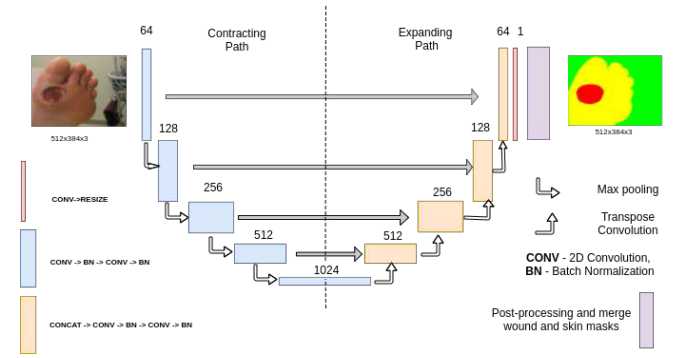
FIGURE 6: Architecture of U-Net.
