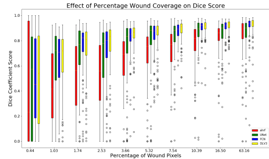
FIGURE 12: Box plot of wound percentage vs dice coefficient for dataset 3
